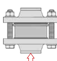
Upwards flow
